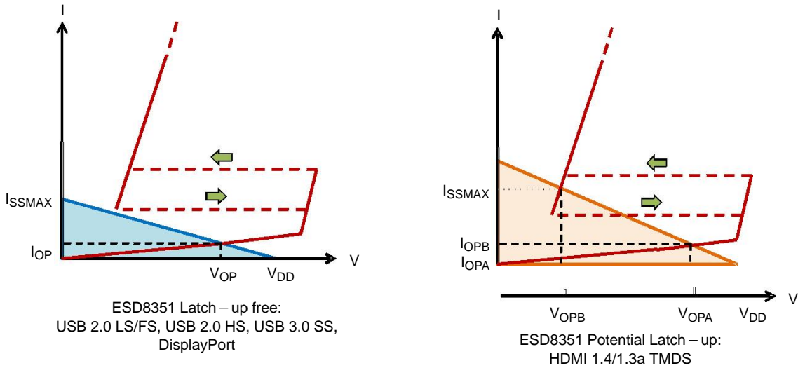
Figure 6. Example Load Lines for Latch-up Free Applications and Applications with the Potential for Latch-up
